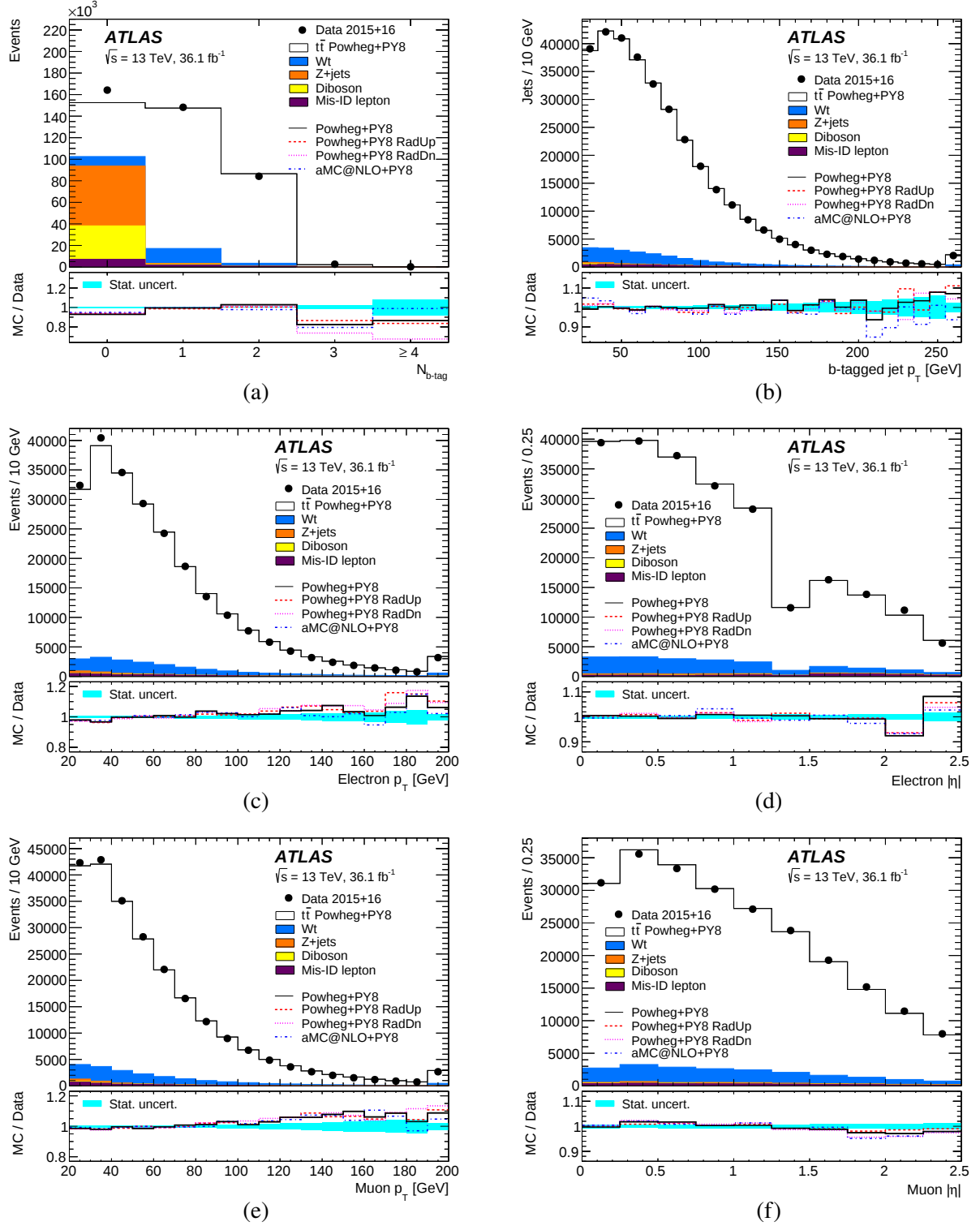
Figure 1: Distributions of (a) the number of b -tagged jets in selected opposite-sign e\mu events; and (b) the p_T of b -tagged jets, (c) the p_T of the electron, (d) the |\eta| of the electron, (e) the p_T of the muon and (f) the |\eta| of the muon, in events with an opposite-sign e\mu pair and at least one b -tagged jet. The reconstruction-level data are compared with the expectation from simulation, broken down into contributions from t\bar{t} (Powheg + PYTHIA8), Wt , Z +jets, dibosons, and events with misidentified electrons or muons. The simulation prediction is normalised to the same integrated luminosity as the data in (a) and to the same number of entries as the data in (b–f). The lower parts of the figure show the ratios of simulation to data, using various t\bar{t} signal samples and with the cyan shaded band indicating the data statistical uncertainty. The last bin includes the overflow in panels (b), (c) and (e).
